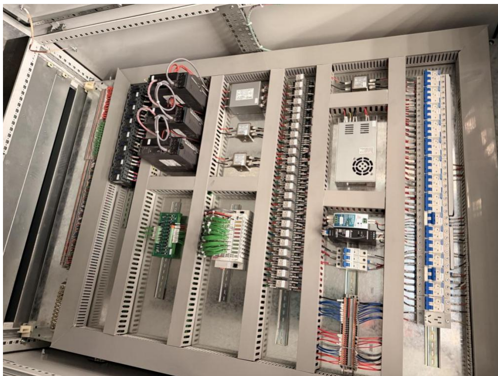
Electrical control cabinet
